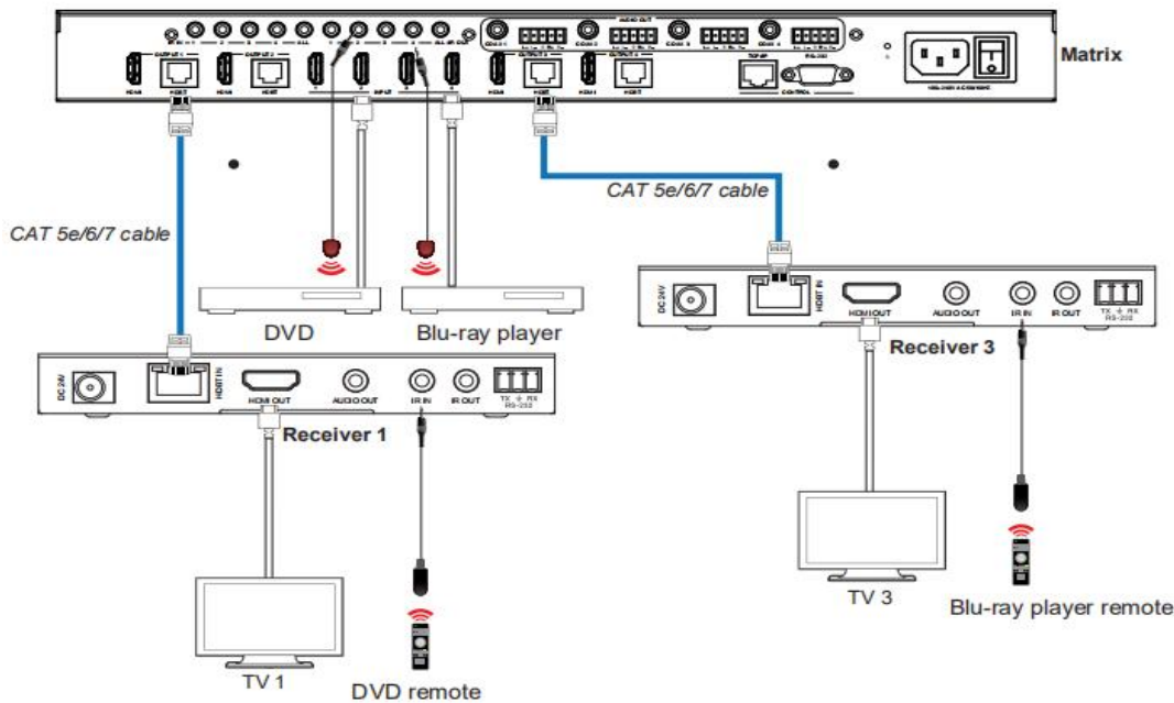
Figure 2: IR connection diagram (HDBaseT Receiver end)
