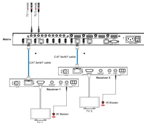
Figure 1: IR connection diagram (Matrix end)
